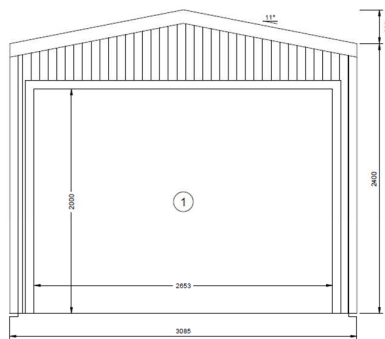
2 FRONT ELEVATION 3 SCALE: 1:25 FRAME #1
