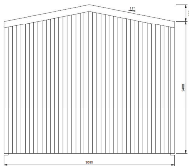
1 REAR ELEVATION 3 SCALE: 1:25 FRAME #2
